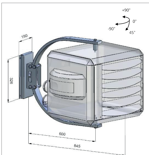
Figure 7 - Adaptateur de suspension
