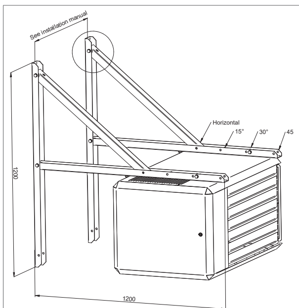
Figure 8 - Support mural (standard)
