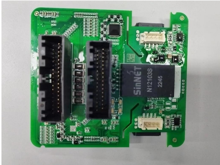
Front view of BMU board
