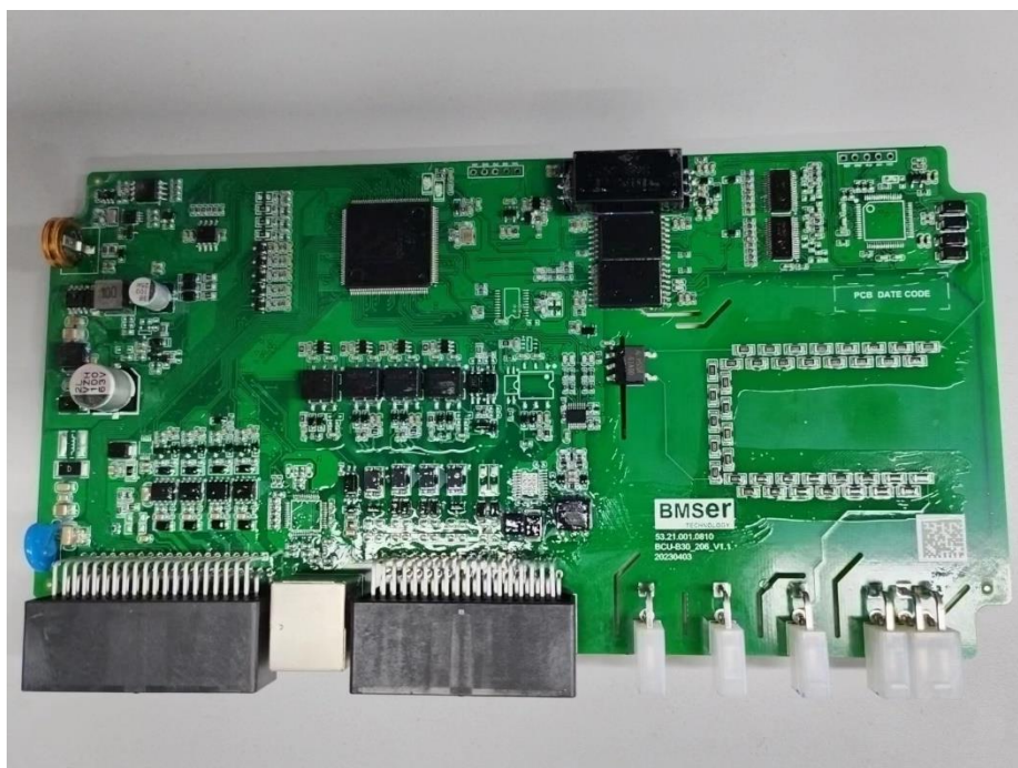
Front view of BCU board
