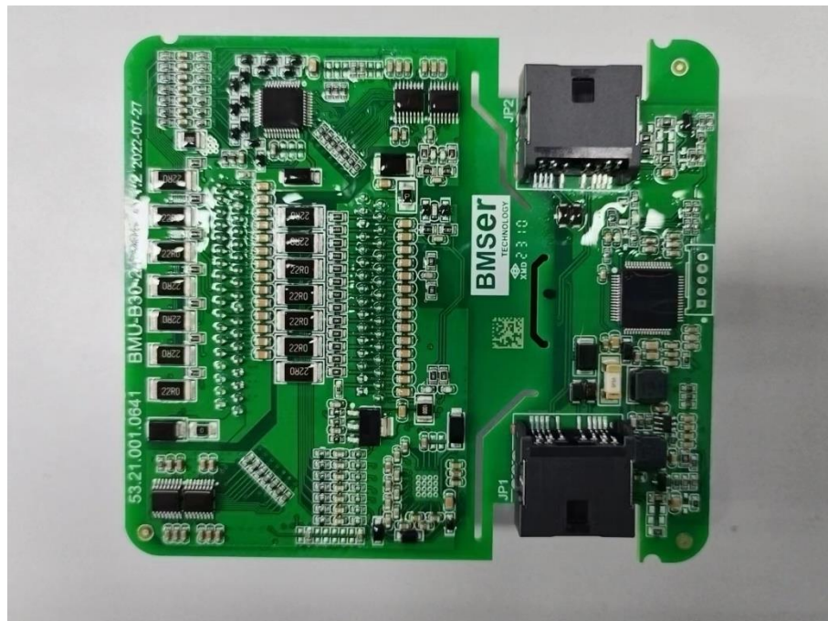
Back view of BMU board
